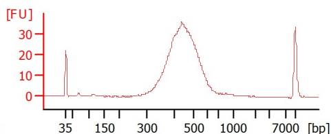
SCN_RGDMH Library
