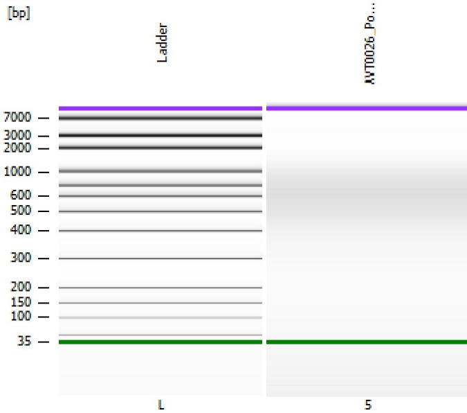
AVT0026_Pooled Libs
