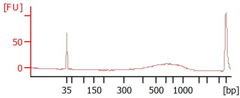
AVT0026_Pooled Libs
