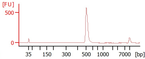
PB941_02_DPM03_Amplicon QC
