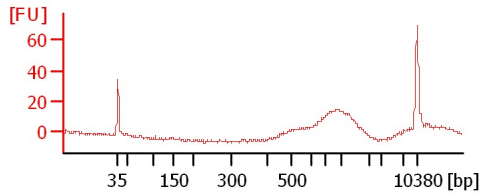
H290P denatured
