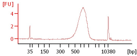
LF7_deltaR Library (1:3)
