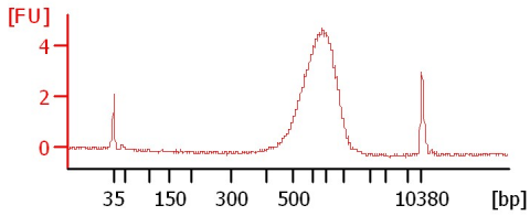
LF7_WT Library (1:3)
