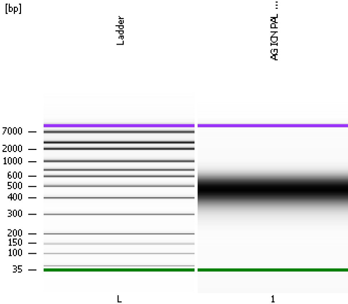
AG ICN PAL 0.68X BC
