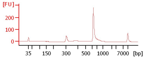
BifSeq&SME amplicon QC (1:70)
