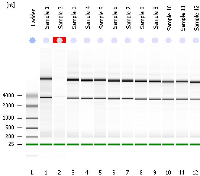
Sample 1 RIN: 8.50
