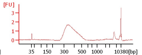
library_fullconc
