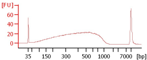
TSA-1 Soni 1:10
