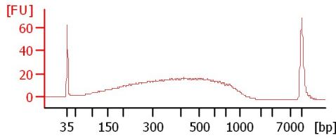
WWI Soni 1:10
