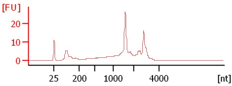
Sample 4 RIN: 7.30
