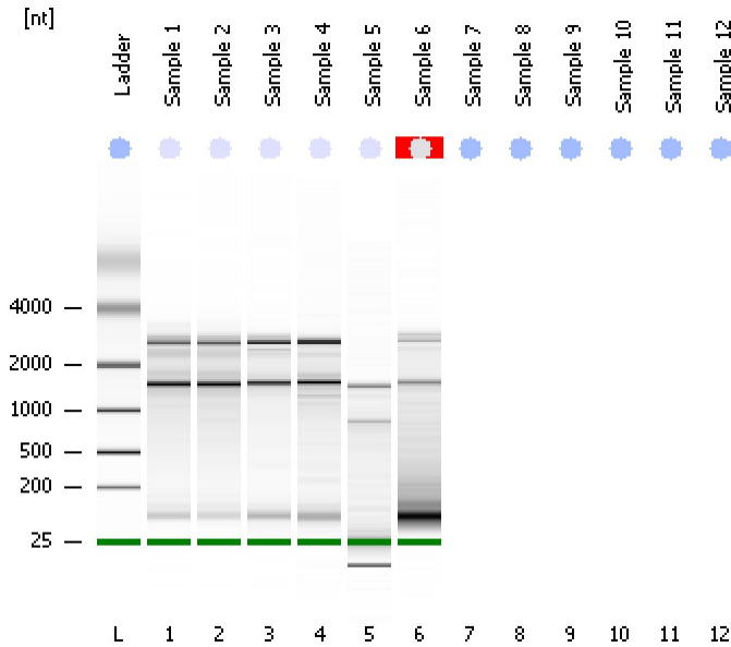
Sample 1 RIN: 7.30
